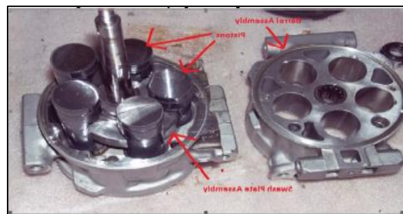
Fig 1: Five cylinder Swash Plate Reciprocating Compressor
